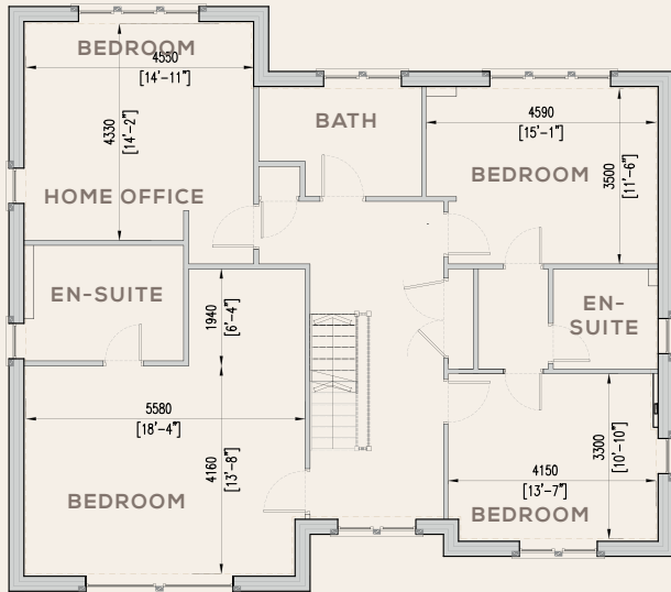
Plot 4 FIRST FLOOR
