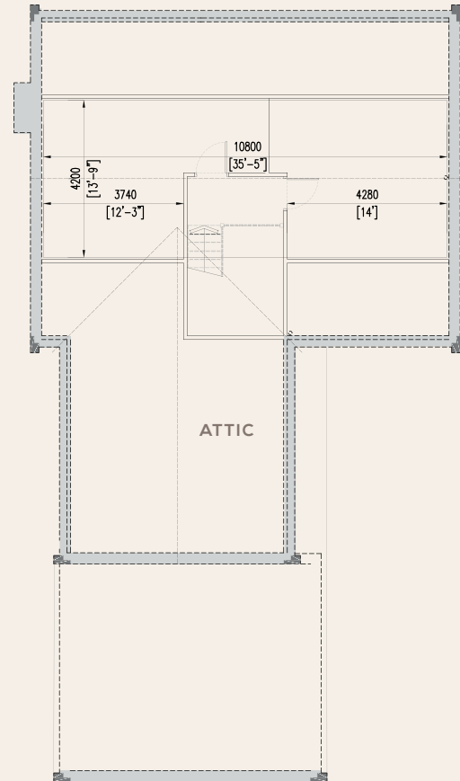
Plot 3 SECOND FLOOR
