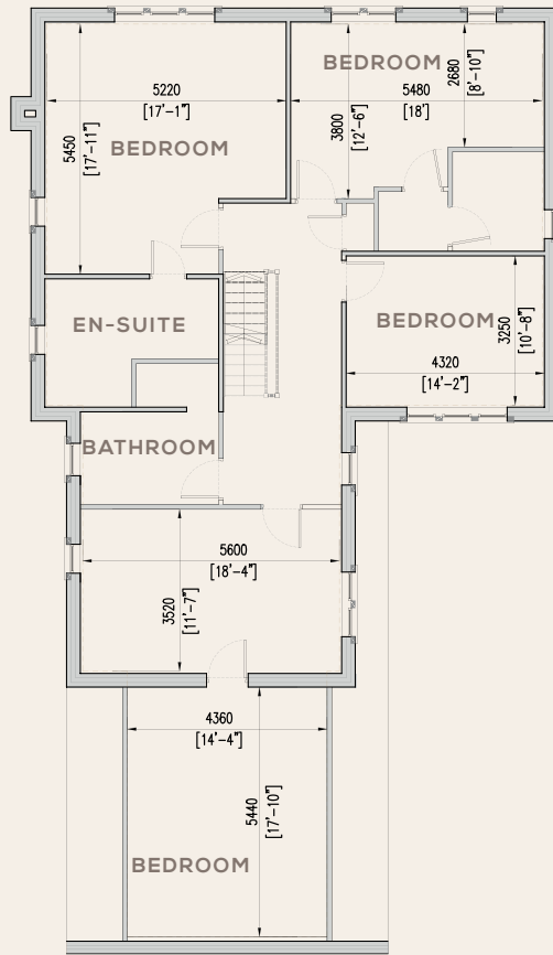
Plot 3 FIRST FLOOR
